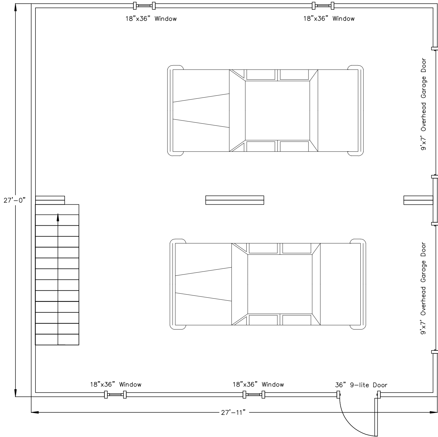
28'x28' TWO STORY DOUBLEWIDE GARAGE
